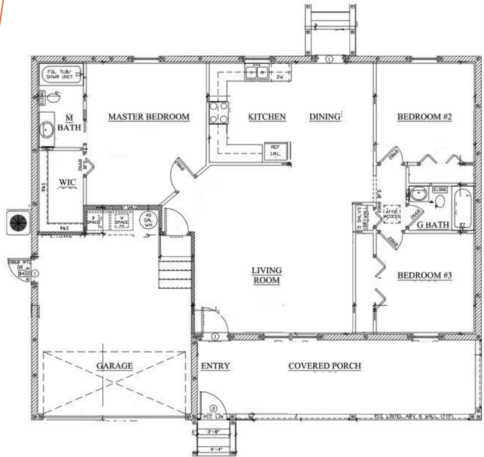
FLOOR PLAN
